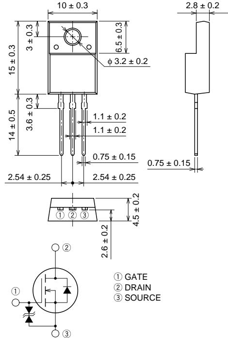
TO-220FN
