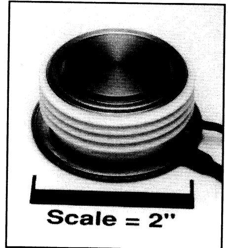
C440 Phase Control SCR 900 Amperes Average, 1600 Volts
