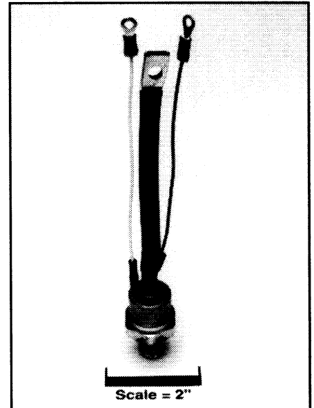
T510 Phase Control SCR 50-80 Amperes (80-125 RMS), 600 Volts
