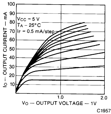
Fig. 1. DC Transfer Characteristics
