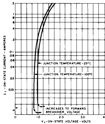
Figure 12. On-State Characteristics
