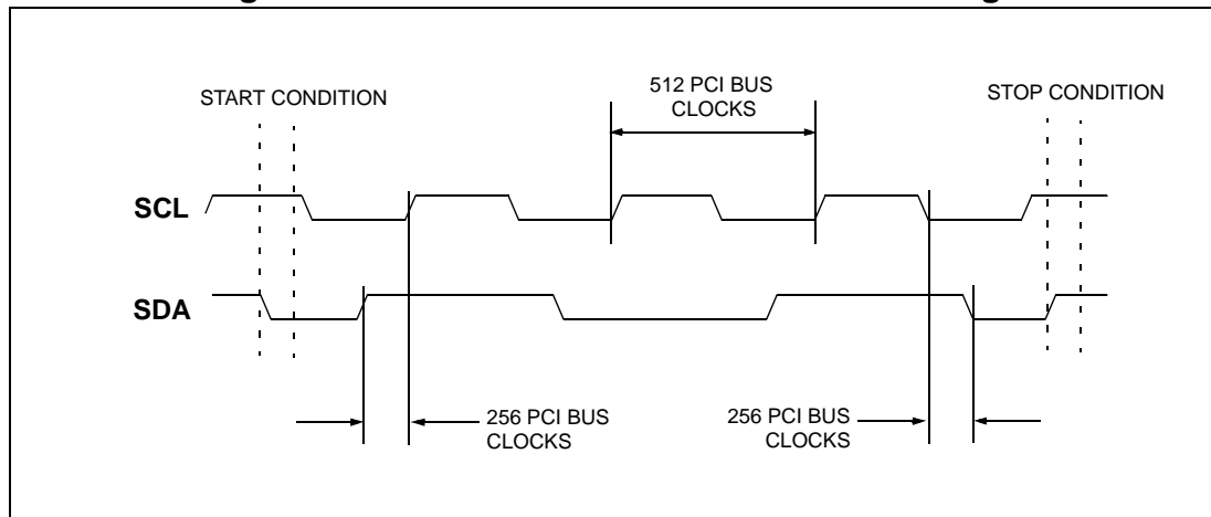
Figure 4: Serial EEPROM Waveforms and Timings
