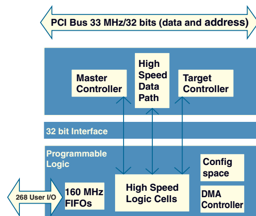
Figure 1: 5732 Block Diagram
