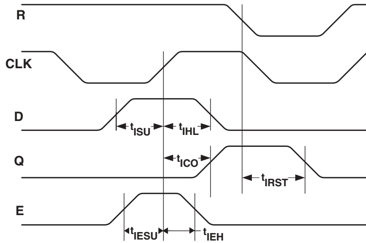
Figure 15: Input Register Cell
