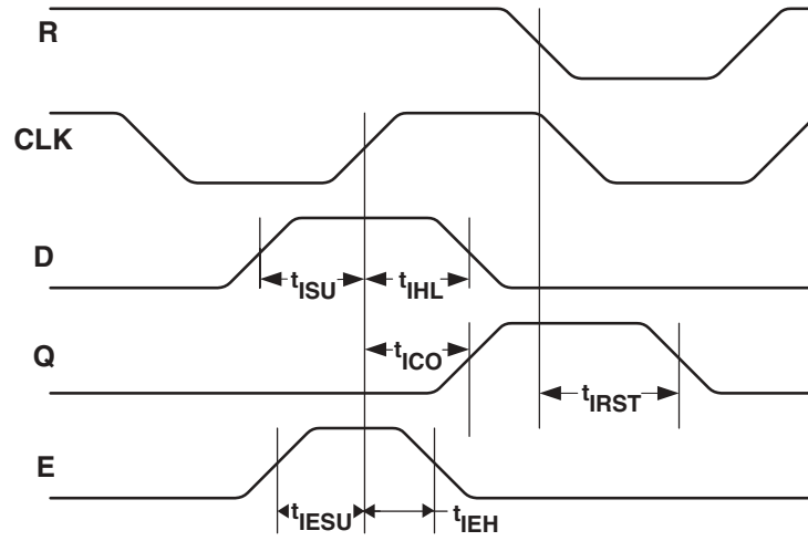
Figure 16: Input Register Cell Timing
