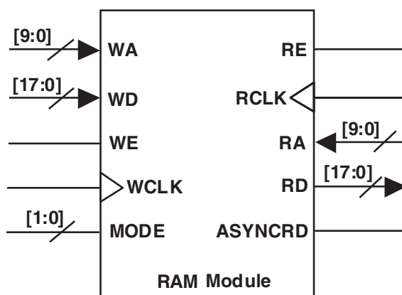
Figure 12: RAM Module
