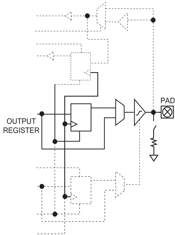
Figure 19: Output Register Cell
