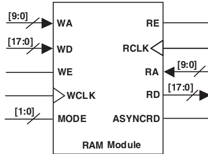
Figure 4: RAM Module
