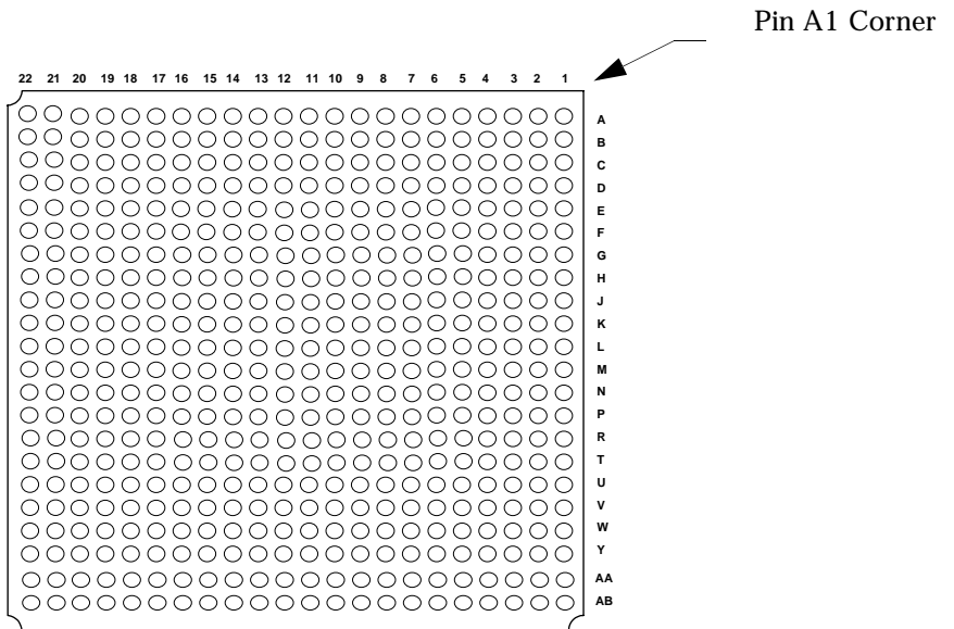
Figure 23: 484 PBGA Pinout Diagram
