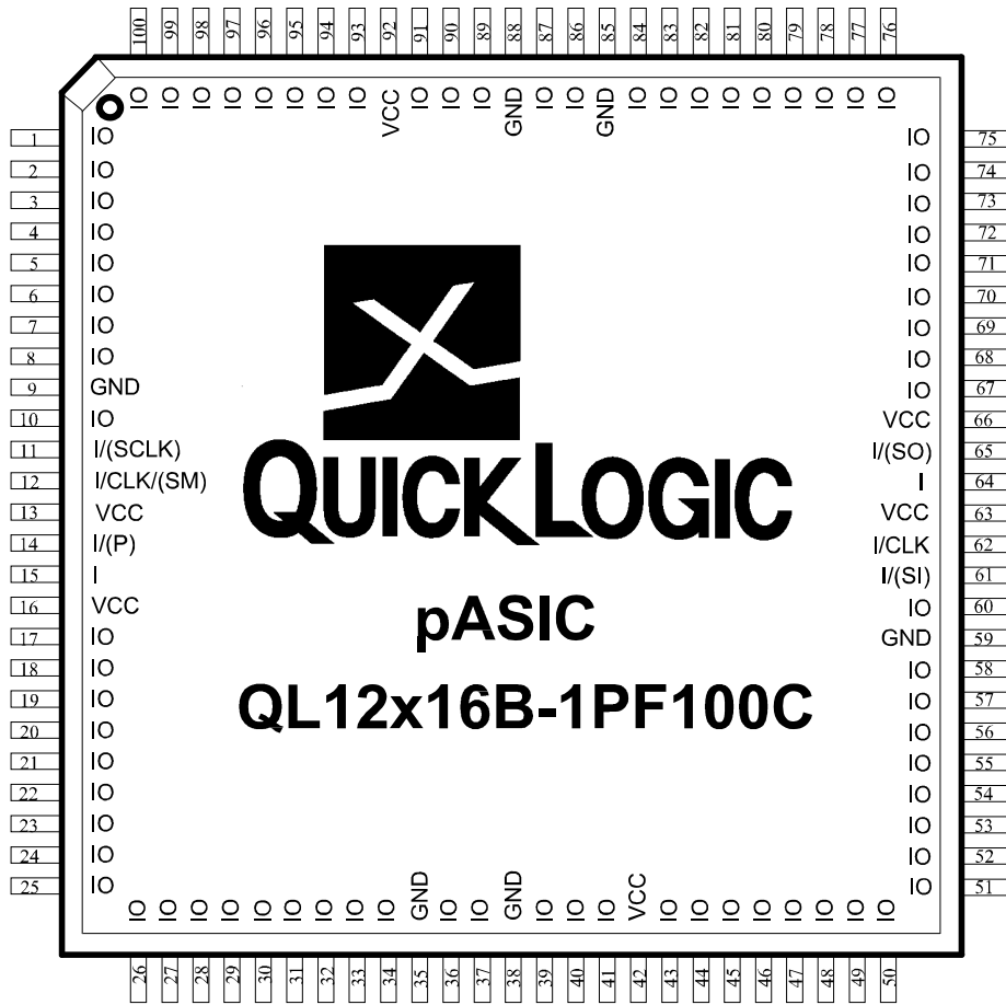
Pinout Diagram 100-pin TQFP
