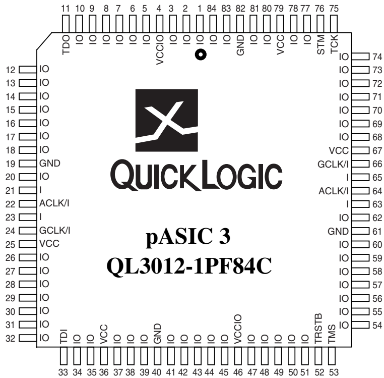
Figure 8: Top View of 84 Pin PLCC
