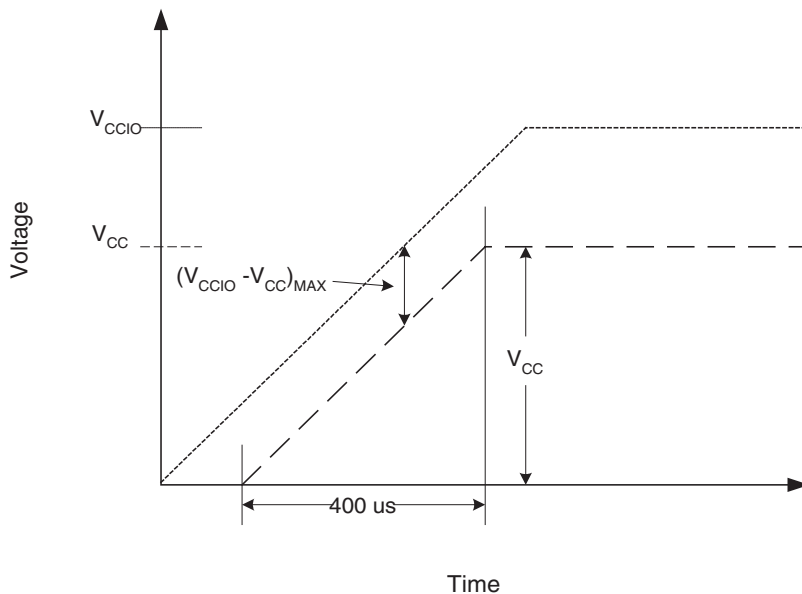
Figure 8: Power-up Requirements
