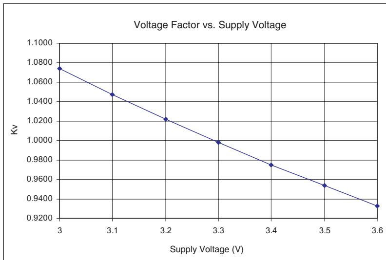
Figure 6: Voltage Factor vs. Supply Voltage
