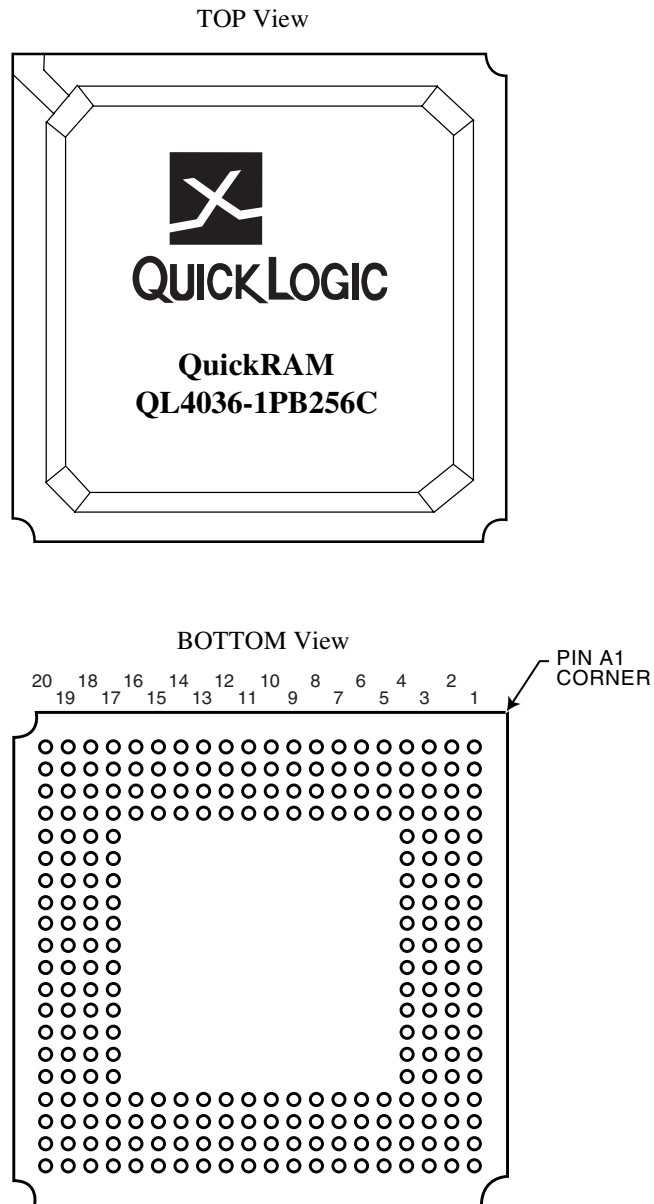
Figure 13: 256 PBGA Pinout Diagram
