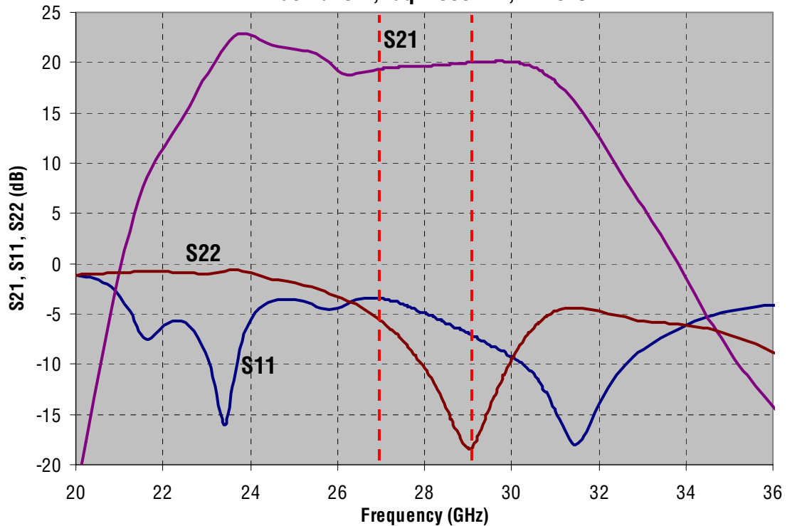
RMPA27000 S21, S11, S22 Mag Vs. Frequency Bias V_d=5 V, I_{dq}=1500 mA, T=25^\circ\text{C}
