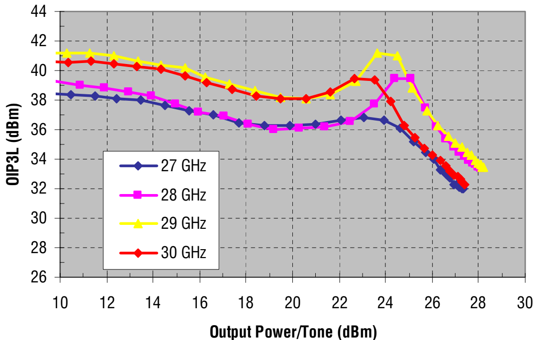
RMPA27000 Two-Tone OIP3 Vs. Output Power /Tone Vd=5V Idq=1500mA T=25°C
