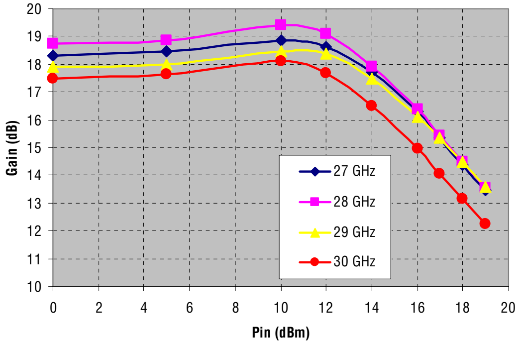
RMPA27000 Gain Vs. Power In Vd=5V Idq=1500mA T=25°C
