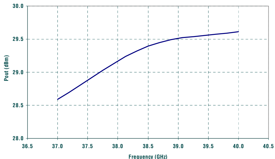
RMPA39000 Saturated Pout Vs. Frequency V_d=5V , I_d=700mA
