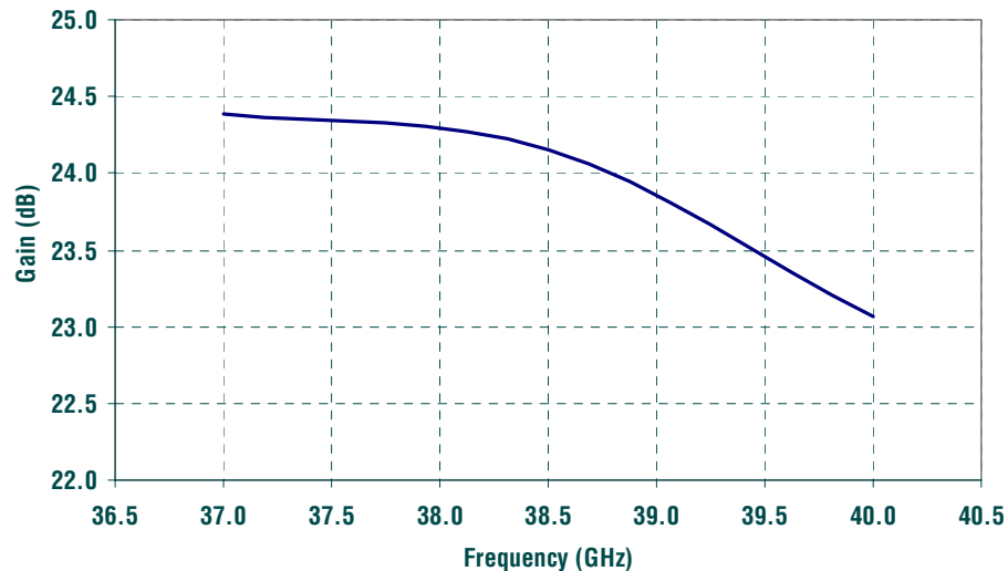
RMPA39000 Gain Vs. Frequency V_d=5V , I_d=700mA
