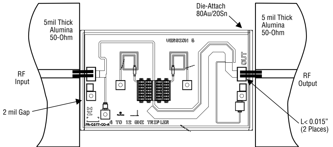
Figure 3 Recommended Assembly Diagram
