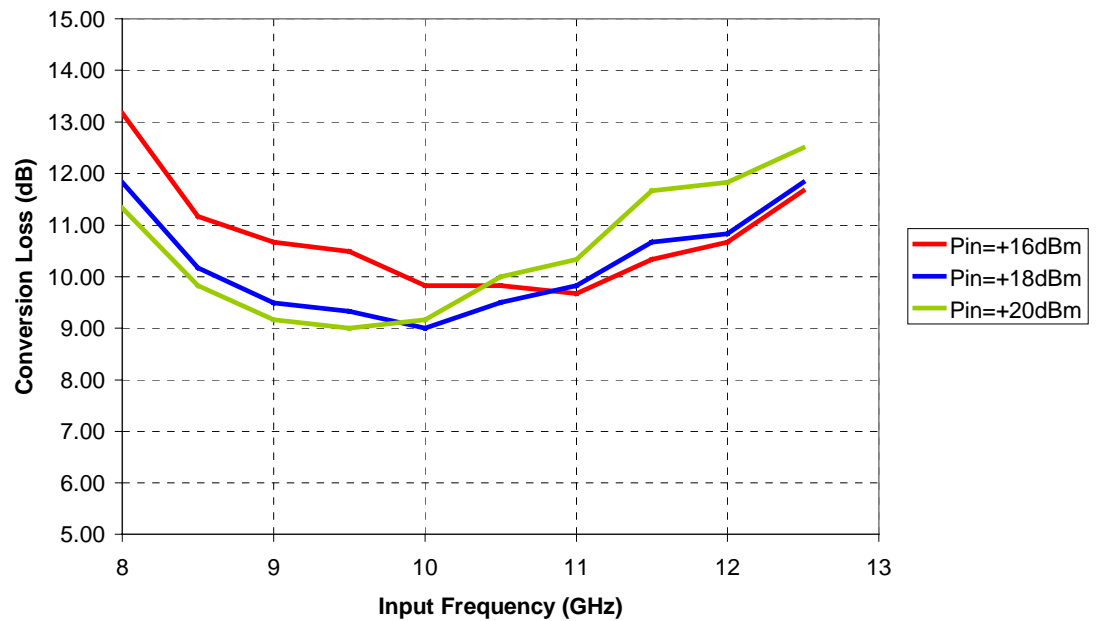
Typical performance, Chip Bonded into 50 ohm Test Fixture
