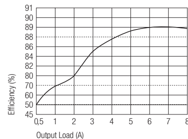
RP40-4805SE Efficiency vs Output Load
