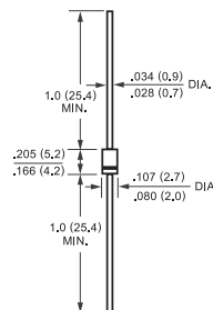
Dimensions in inches and (millimeters)
