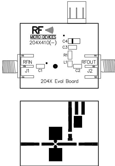
Evaluation Board Layout Board Size 1.195" x 1.000"
