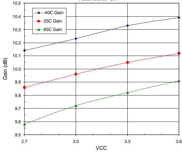
LNA Gain versus VCC (2.45 GHz), Attenuator On
