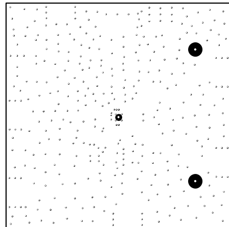
Power Plane 2
