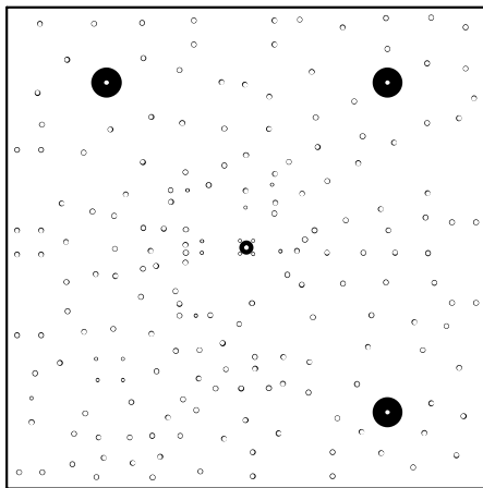
Power Plane
