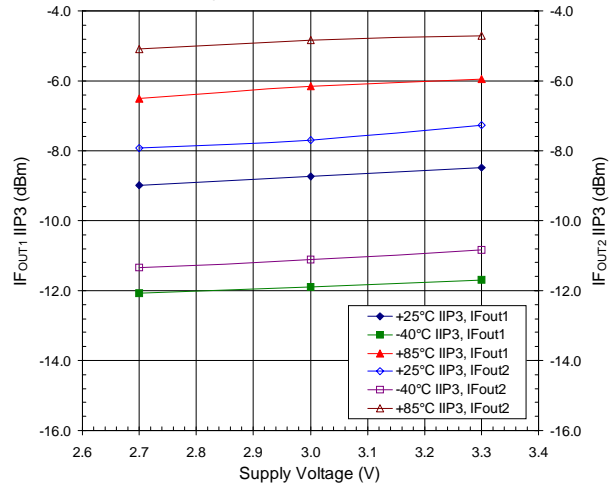
LNA1+Mixer1 Input IP3 versus Supply Voltage
