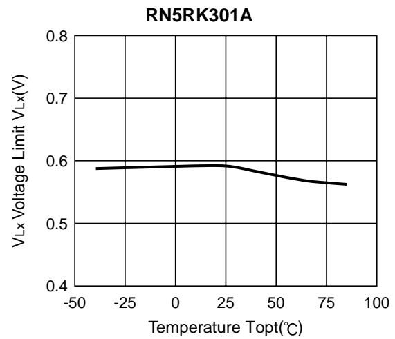
16) VLX Voltage Limit vs. Temperature
