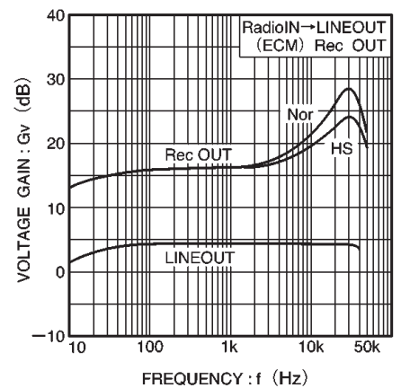
Fig. 6 Voltage gain vs. frequency
