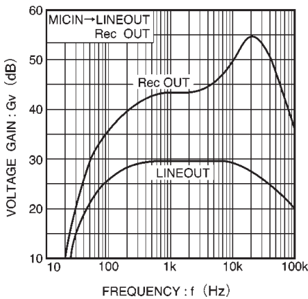
Fig. 7 Voltage gain vs. frequency
