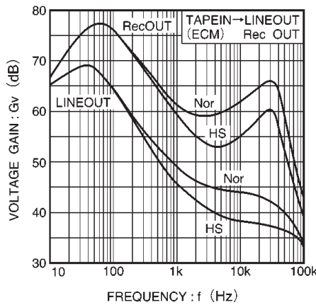
Fig. 8 Voltage gain vs. frequency
