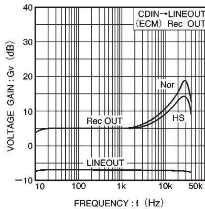
Fig. 5 Voltage gain vs. frequency
