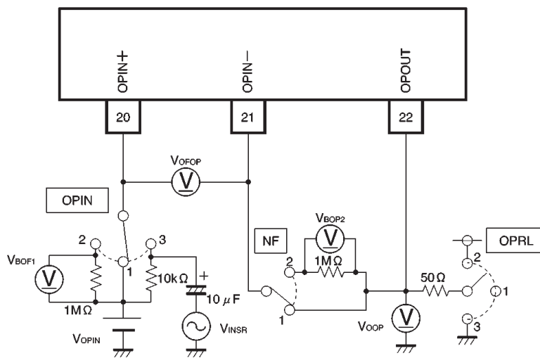
Fig.2 Operational amplifier measurement circuit diagram
