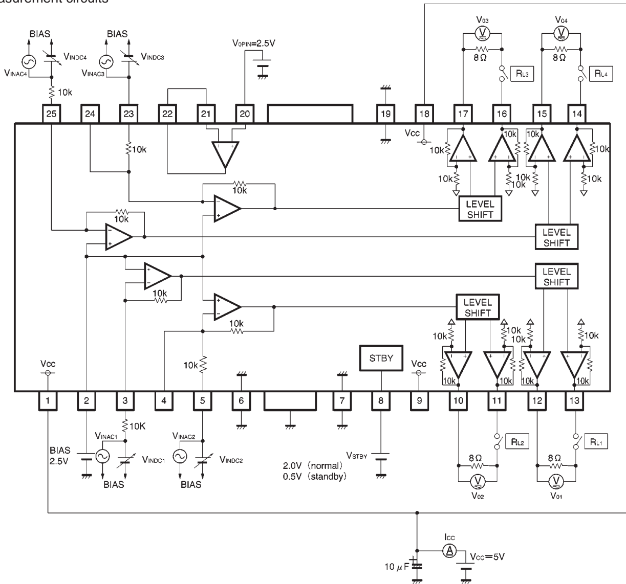
Fig.1 Driver block measurement circuit diagram
