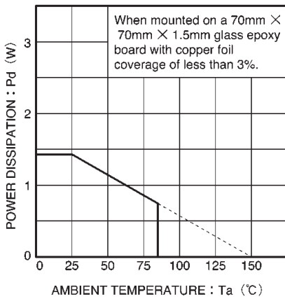
Fig.4 Thermal derating curve
