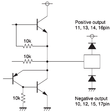
Driver output
