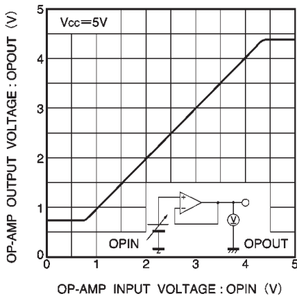
Fig.7 Op-amp I/O characteristics
