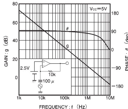
Fig.8 Op-amp open loop characteristics
