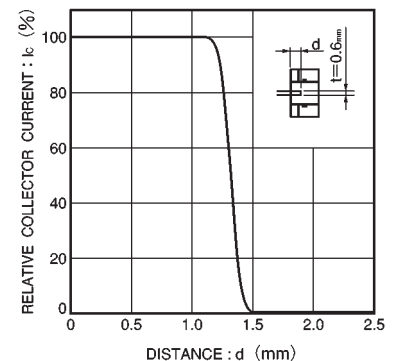
Fig.6 Relative output current vs. distance (1)
