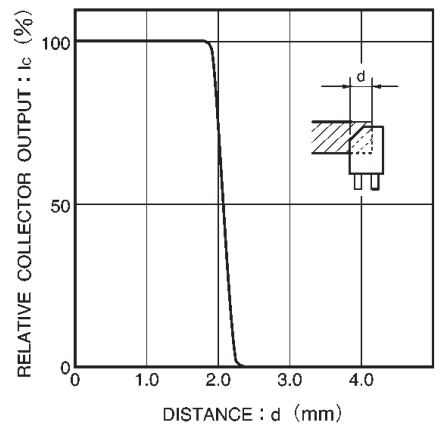
Fig.6 Relative output vs. distance
