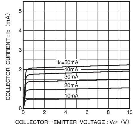
Fig.9 Output characteristics
