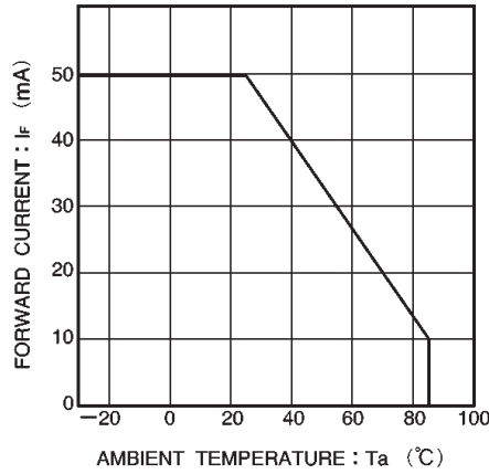
Fig.8 Forward current falloff
