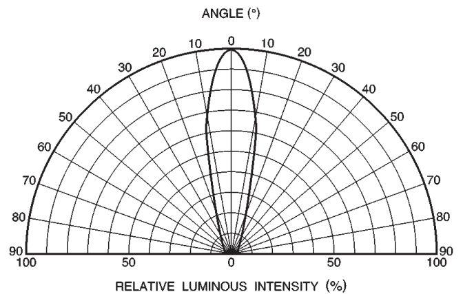
Fig. 3 SLA-370 Directional pattern
