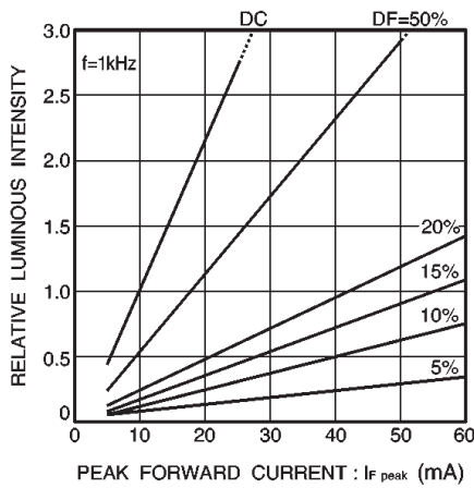
Fig. 14 Luminous intensity vs. peak forward current
