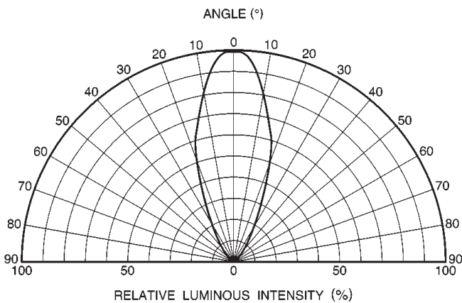
Fig. 2 SLA-360 Directional pattern
