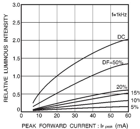
Fig. 8 Luminous intensity vs. peak forward current
