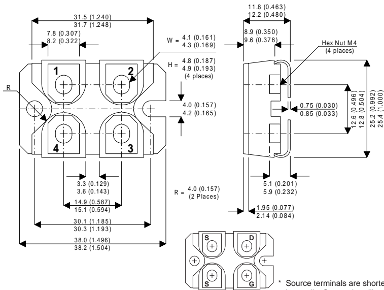
SOT-227 Package Outline. Dimensions in mm (inches)
