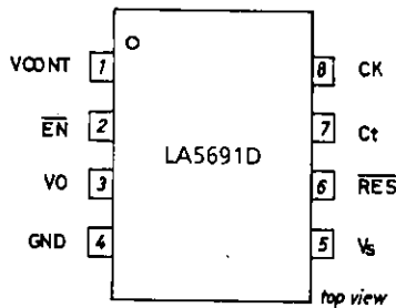
DIP 8
