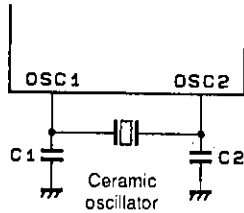
Figure 1 Oscillator Circuit
