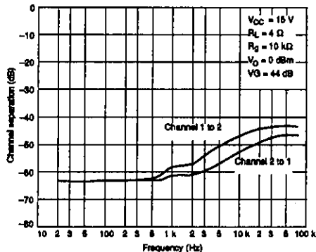
Channel separation vs. frequency
