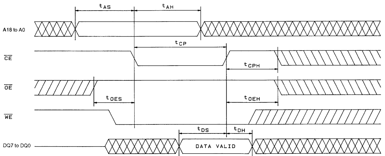
Figure 5 \overline{CE} Control Write Cycle
