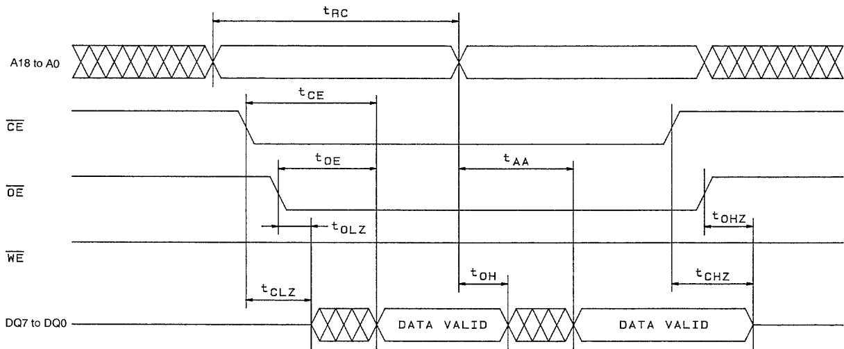
Figure 3 Read Cycle
