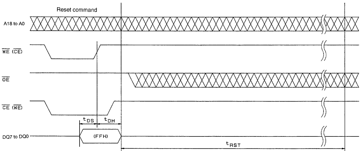
Figure 8 Reset
