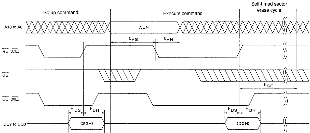
Figure 6 Sector Erase
