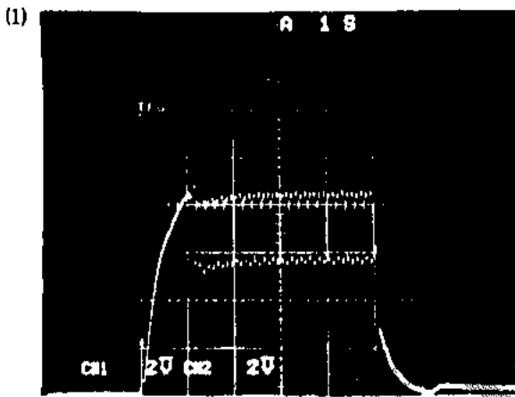
DC GND Main SW ON Main SW OFF
