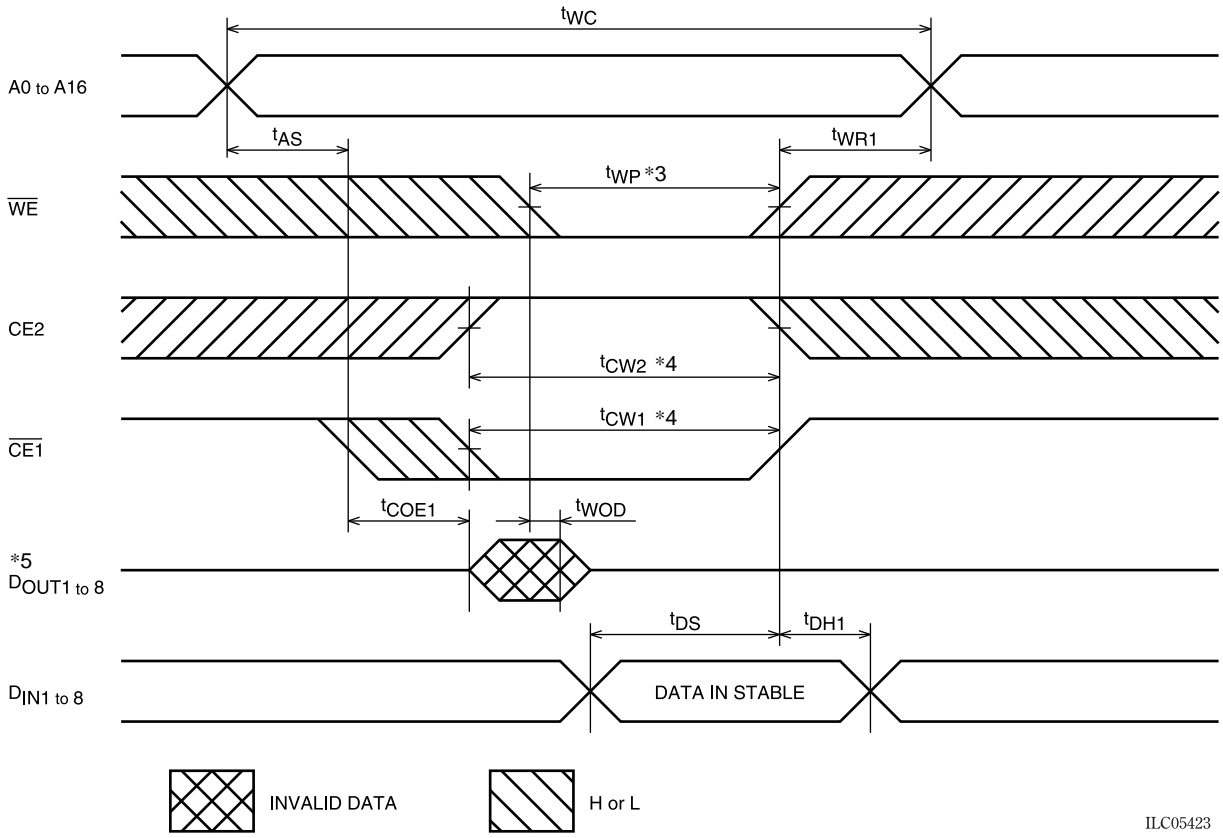
Write cycle (2) ( \overline{\text{CE1}} write)
