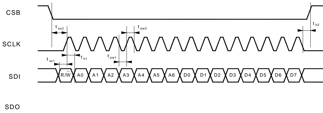
Read access timing in SERIAL Mode.
