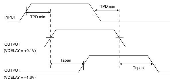
Figure 2. VDELAY Control
