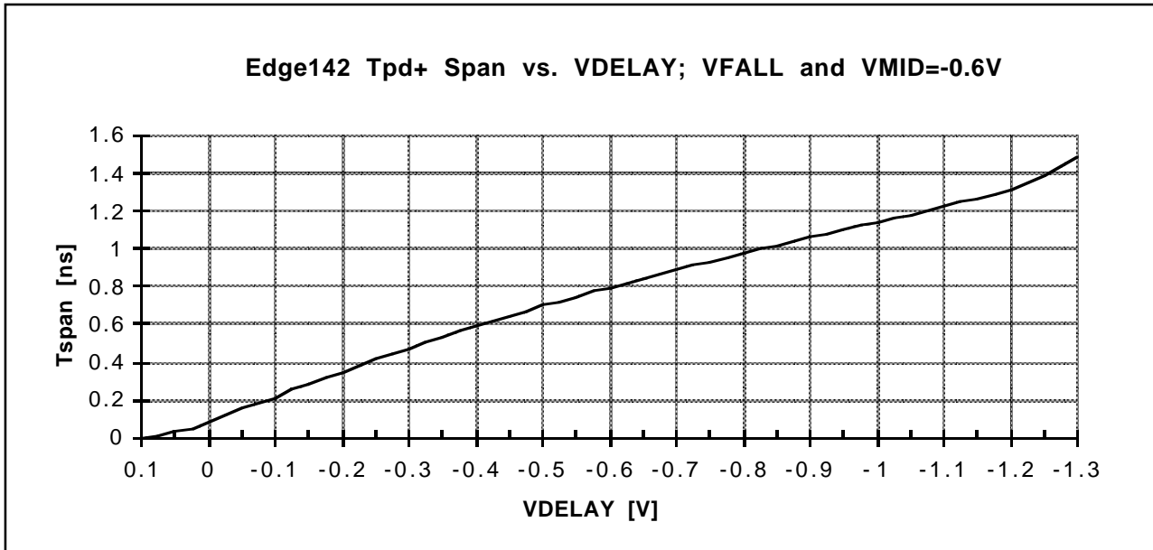
Figure 4. VDELAY Transfer Function
