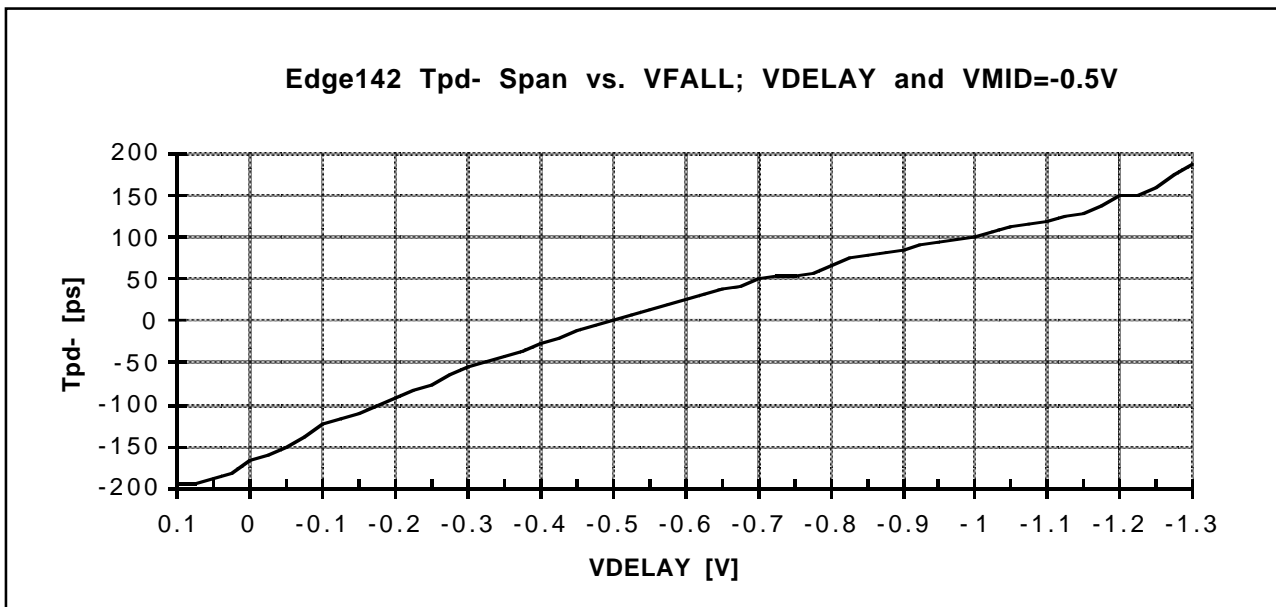
Figure 5. VFALL Transfer Function
