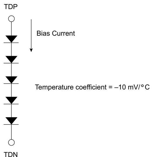
Figure 6. Thermal Diode String
