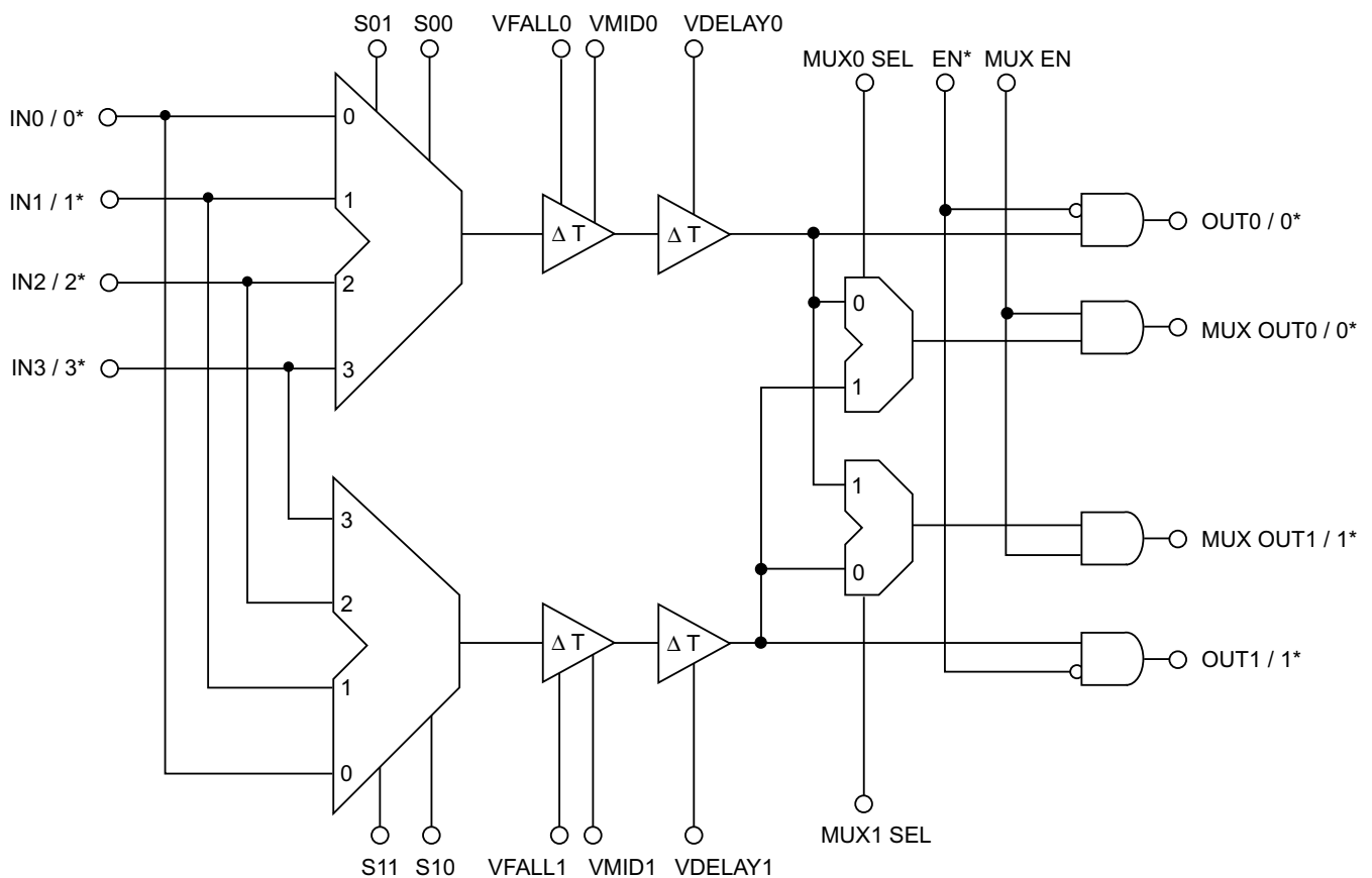
Figure 1. Edge142 Block Diagram
