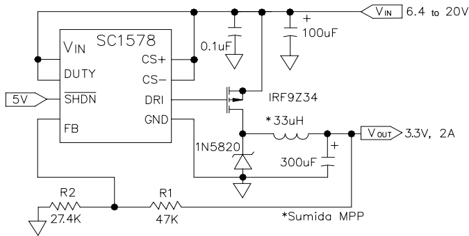
Figure 2. 3.3 Step-Down Converter
