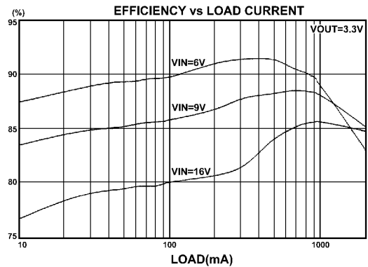
Figure 2. 3.3 Step-Down Converter
