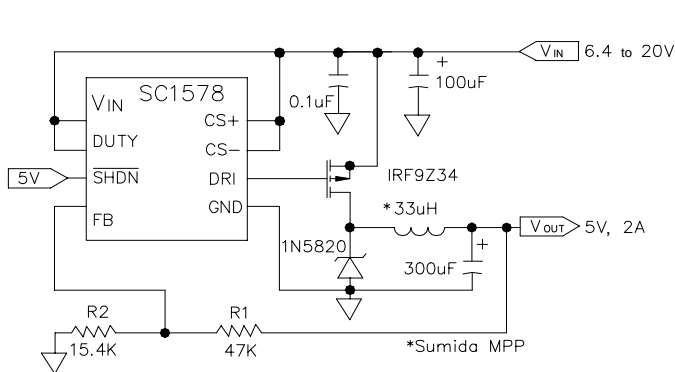
Figure 1. 5V Step-Down Converter
