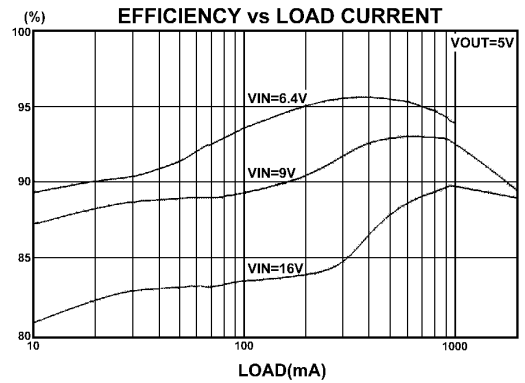
Figure 1. 5V Step-Down Converter
