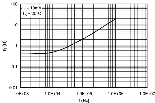
Reference Impedance vs. Frequency
