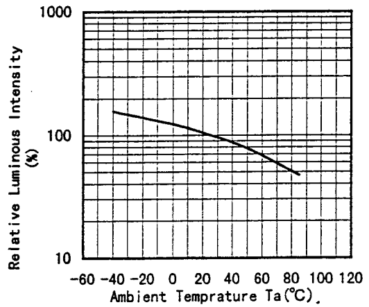
Relative Luminous Intensity vs. Ambient Temperature ( I_F=20\text{mA} )
