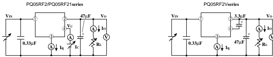
Fig.1 Test Circuit
