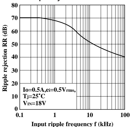
Fig.10 Ripple Rejection vs. Input Ripple Frequency
