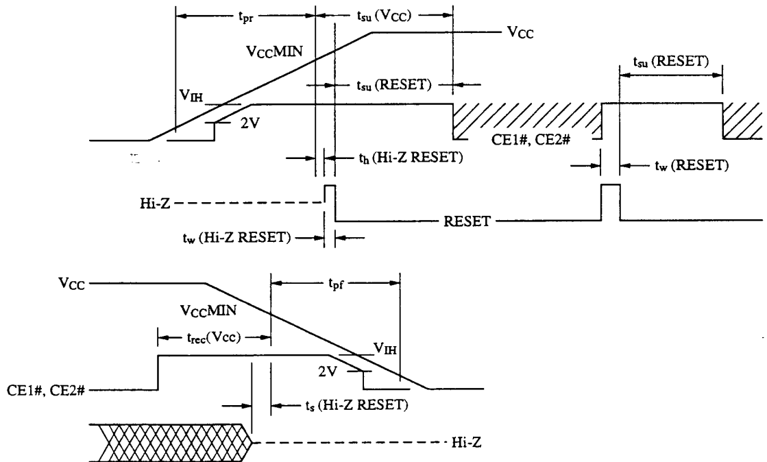
Power-Up/Down Timing fot Systems Supporting RESET
