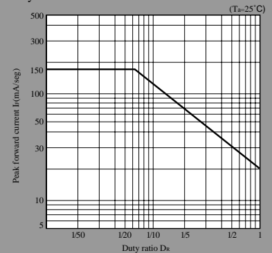
Duty Ratio vs. Peak Forward Current ( T_a=25^\circ\text{C} )
