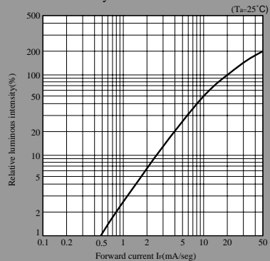
Luminous Intensity vs. Forward Current ( T_a=25^\circ\text{C} )
