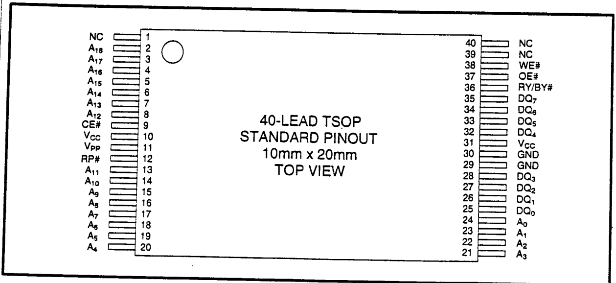
Figure 2. TSOP 40-Lead Pinout
