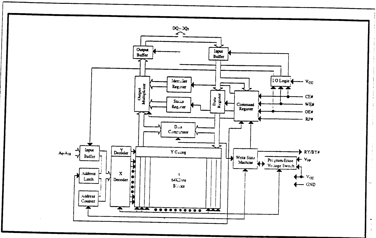
Figure 1. Block Diagram
