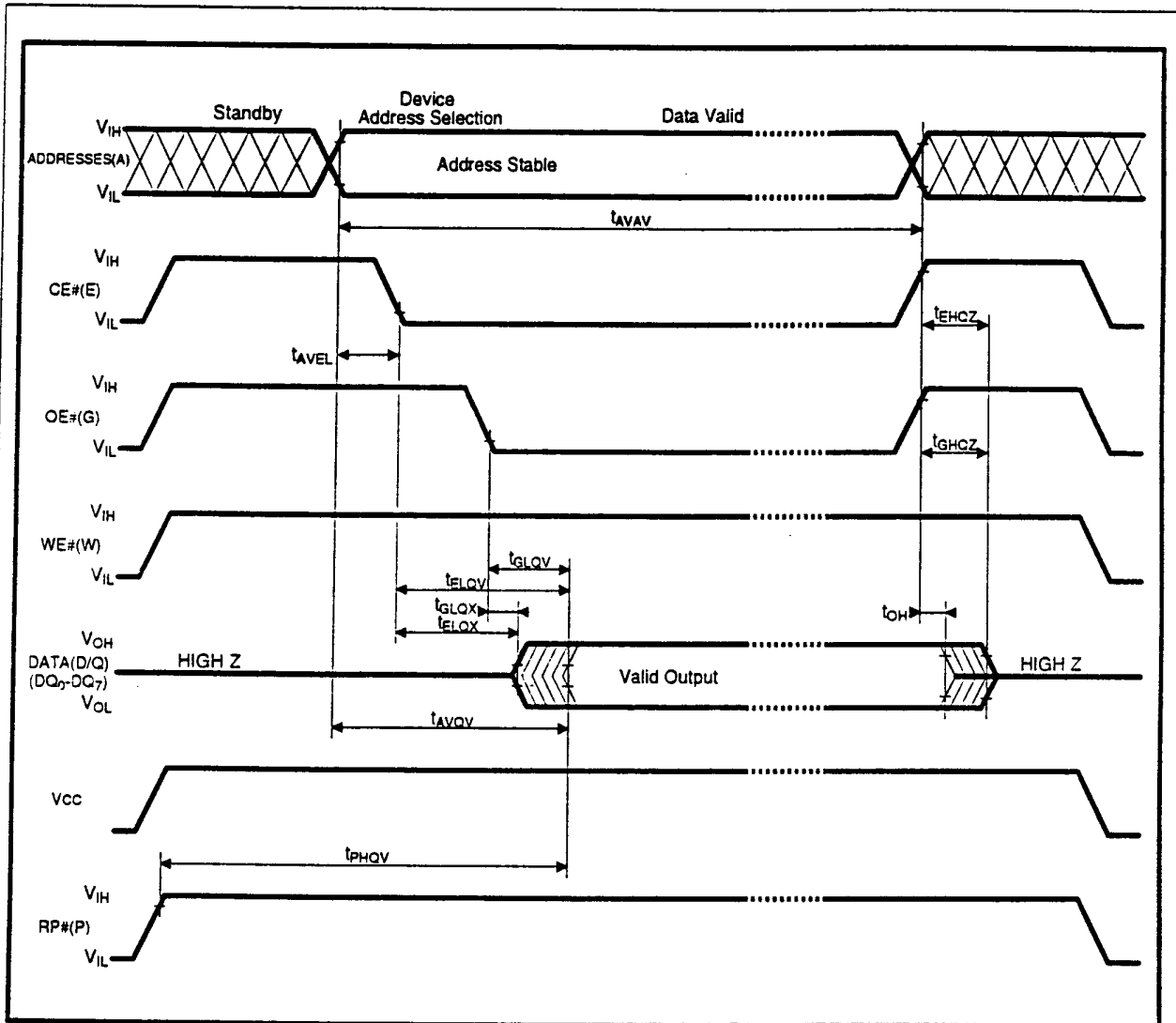
Figure 15. AC Waveform for Read Operations
