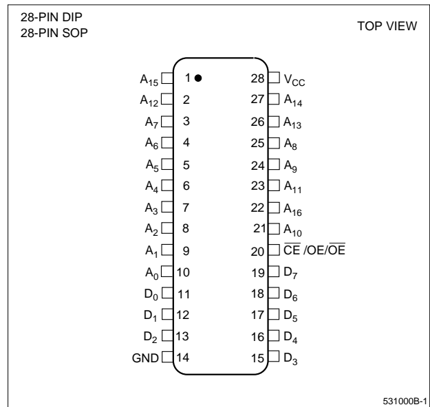
Figure 1. Pin Connections for DIP and SOP Packages
