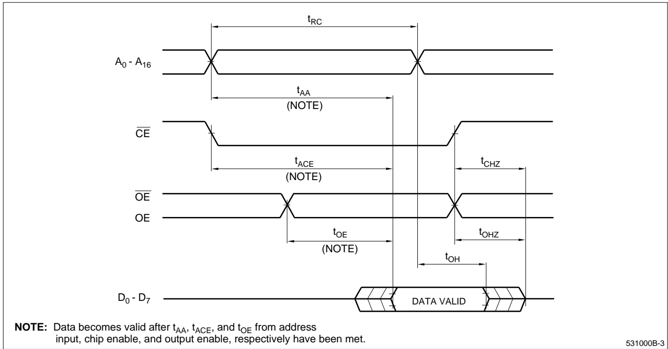
Figure 3. Timing Diagram
