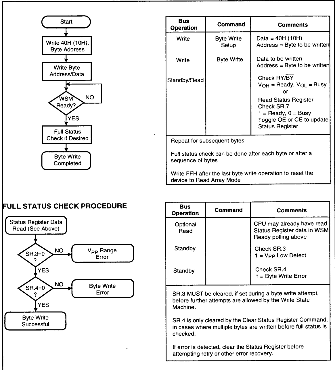
Figure 5. Automated Byte Write Flowchart
