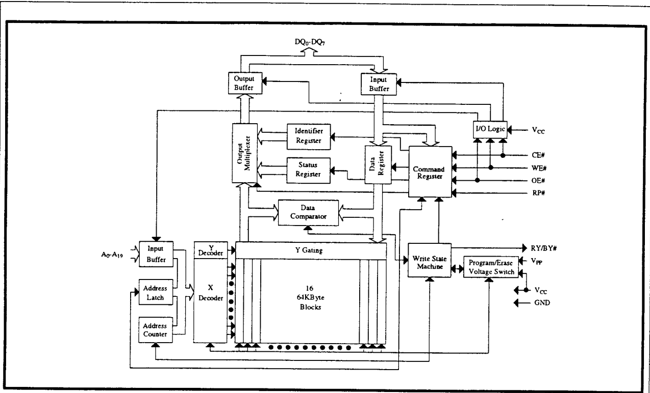
Figure 1. Block Diagram
