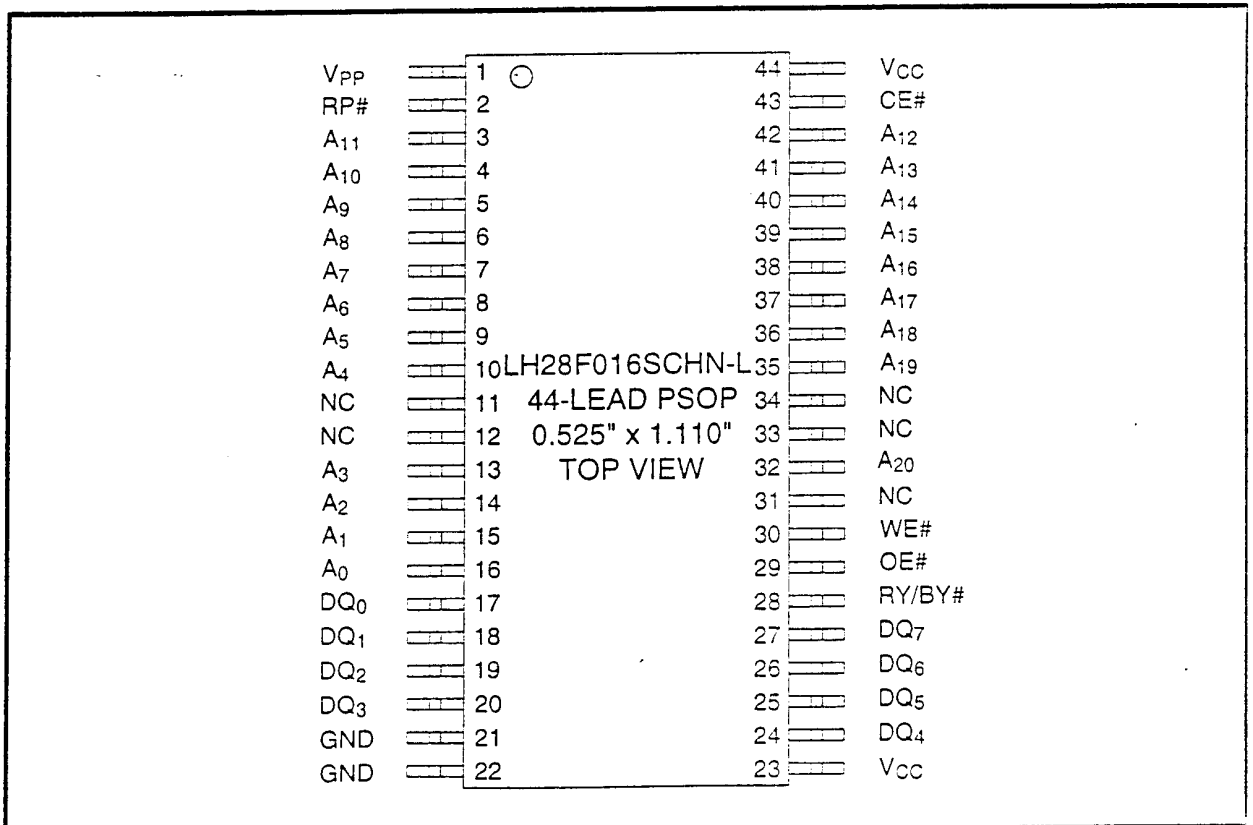
Figure 3. PSOP 44-Lead Pinout
