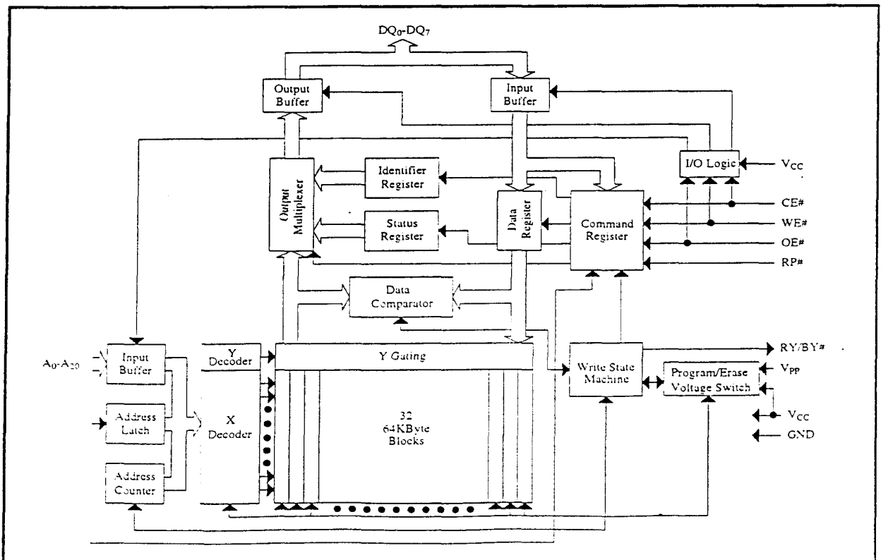
Figure 1. Block Diagram
