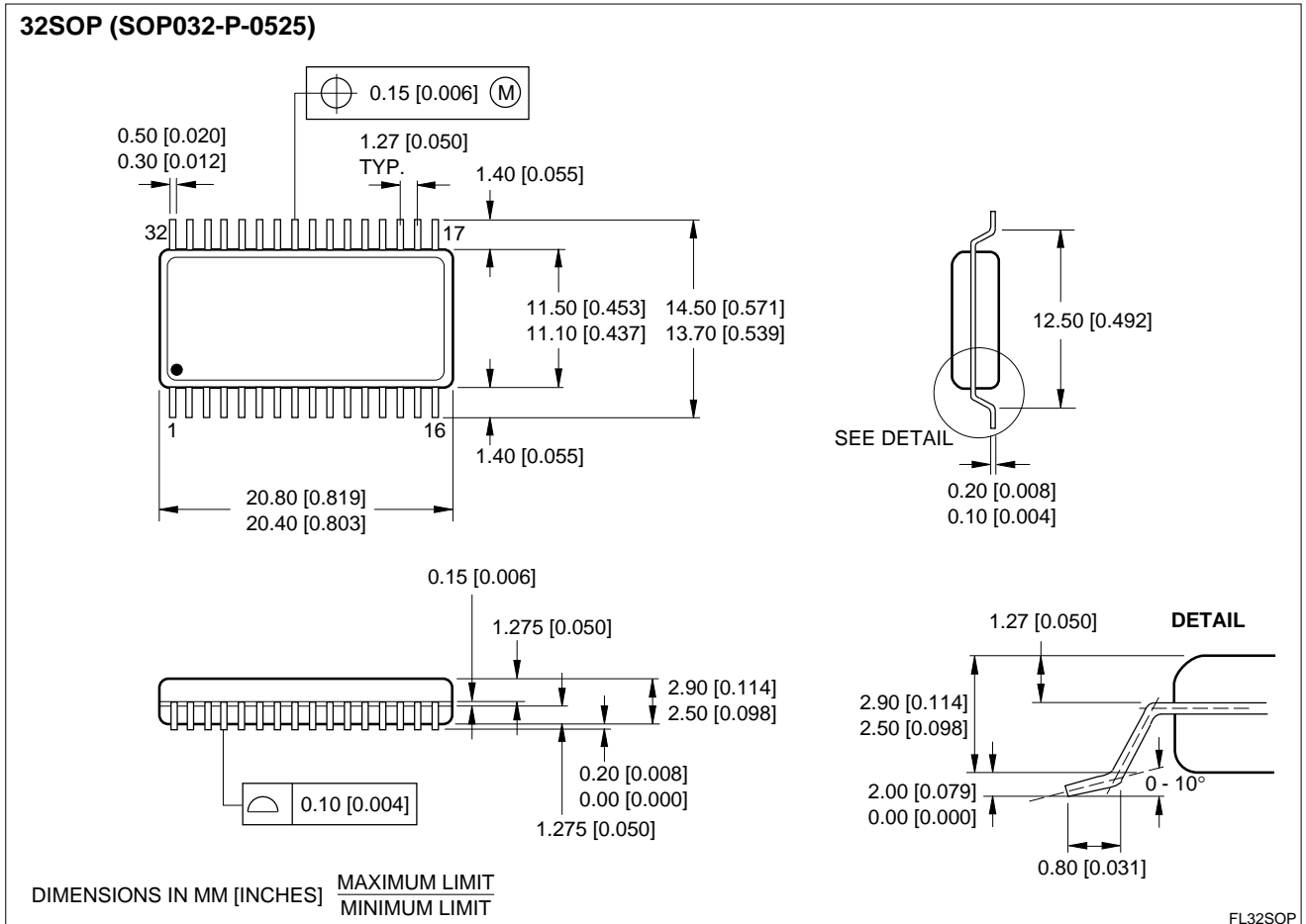
Figure 20. 32-Pin SOP
