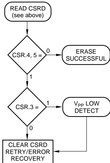
Figure 6. Block Erase with Compatible Status Register
