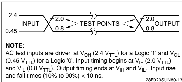
Figure 14. Transient Input/Output Reference Waveform ( V_{CC} = 5.0 V )
