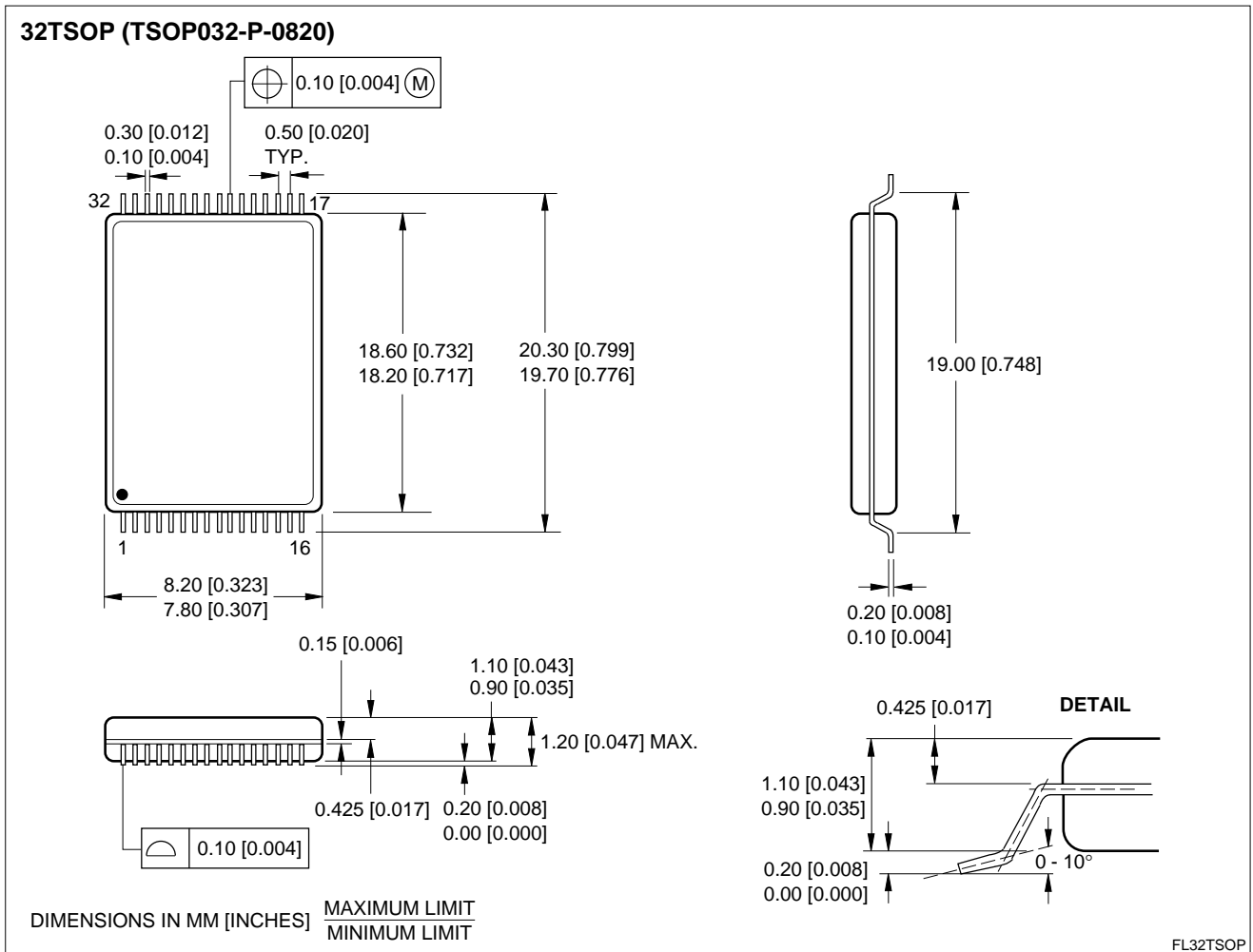
Figure 21. 32-Pin TSOP
