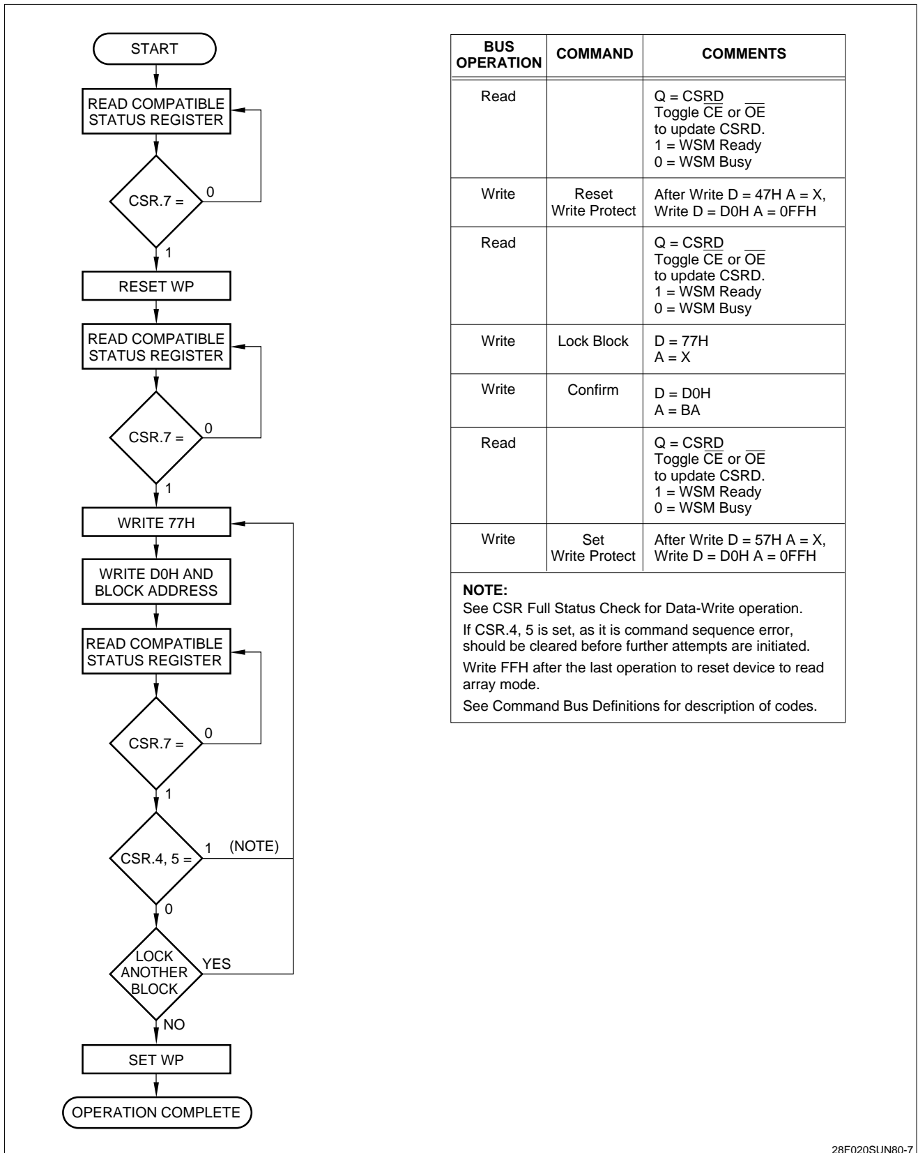
Figure 8. Block Locking
