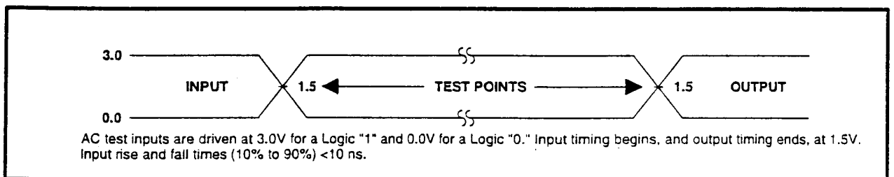
Figure 16. Transient Input/Output Reference Waveform for V_{CC}=3.3V\pm 0.3V
