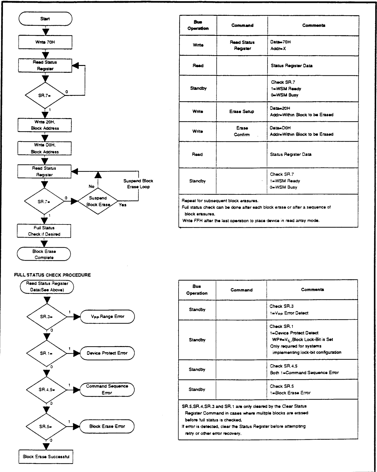
Figure 6. Automated Block Erase Flowchart
