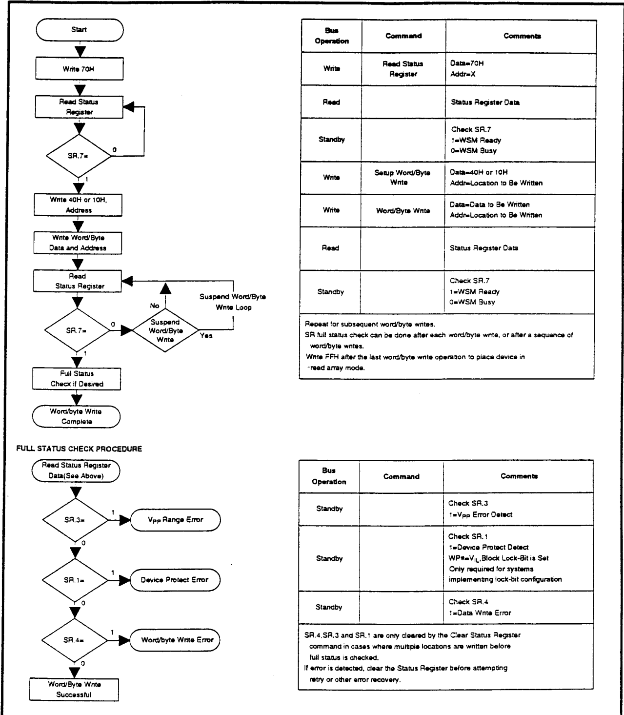
Figure 8. Automated Word/byte Write Flowchart
