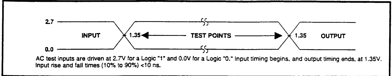
Figure 15. Transient Input/Output Reference Waveform for V_{CC}=2.7V-3.6V
