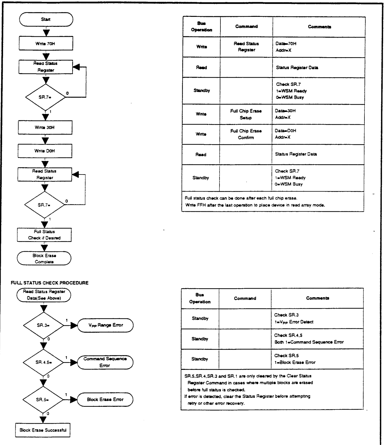
Figure 7. Automated Full Chip Erase Flowchart
